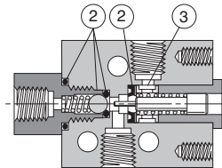
3-Way Poppet
