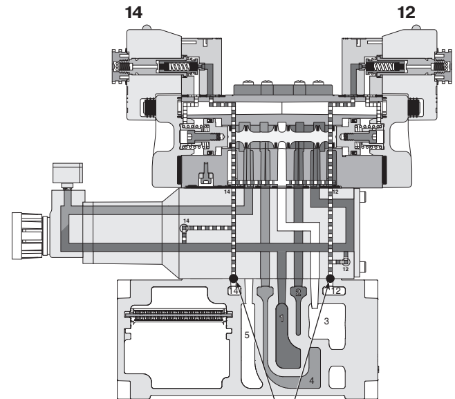
Sandwich Regulator has standard configuration of internal Pilot with the Pilot Plug in the bottom #12 and #14 Pilot Hole which prevents line pressure from escaping through the manifold.
