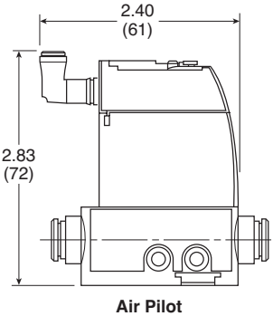
Air Pilot
